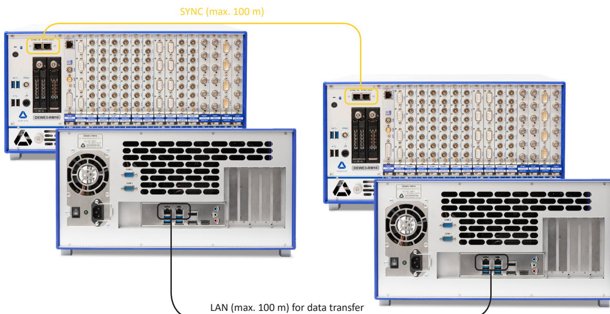
Fig. 24: Network with multiple systems
