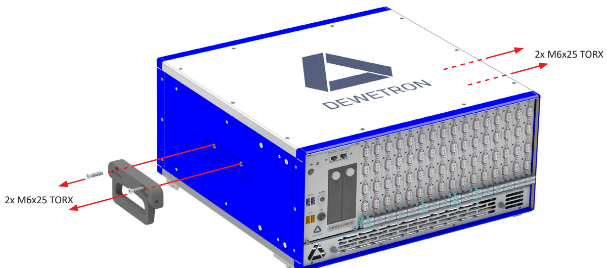
Fig. 9: Demounting the handles
