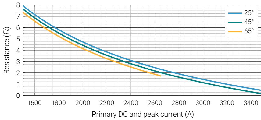
Figure 2: Maximum measurement resistor R_M vs. ambient temperatures
