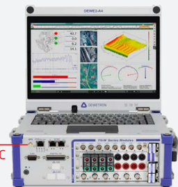
DEWE3-A4 with integrated GPS interface
