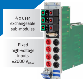
TRION(3)-18xx-POWER
